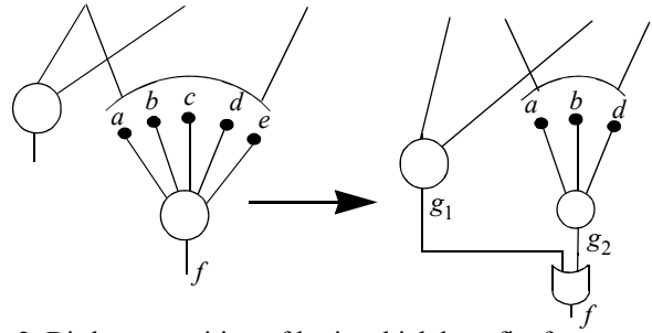
Fig. 2. Bi-decomposition of logic which benefits from re-using existing for g_1 logic.
