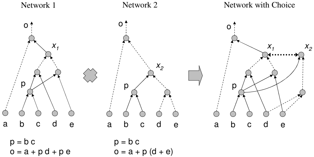
Figure 4: Example illustrating the creation of a network with choices. A choice is created when there are two nodes with the same global function (upto complementation), but different structures. Thus nodes x_1 and x_2 lead to a choice, but node p does not ( p is structurally the same in both networks).
